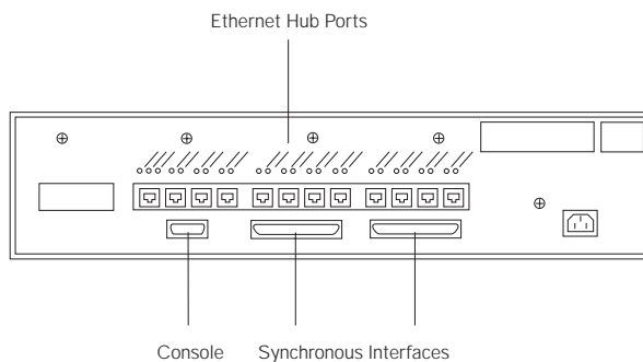
Figure 2 | 2-Port Access Node Router/Hub Connector Panel
